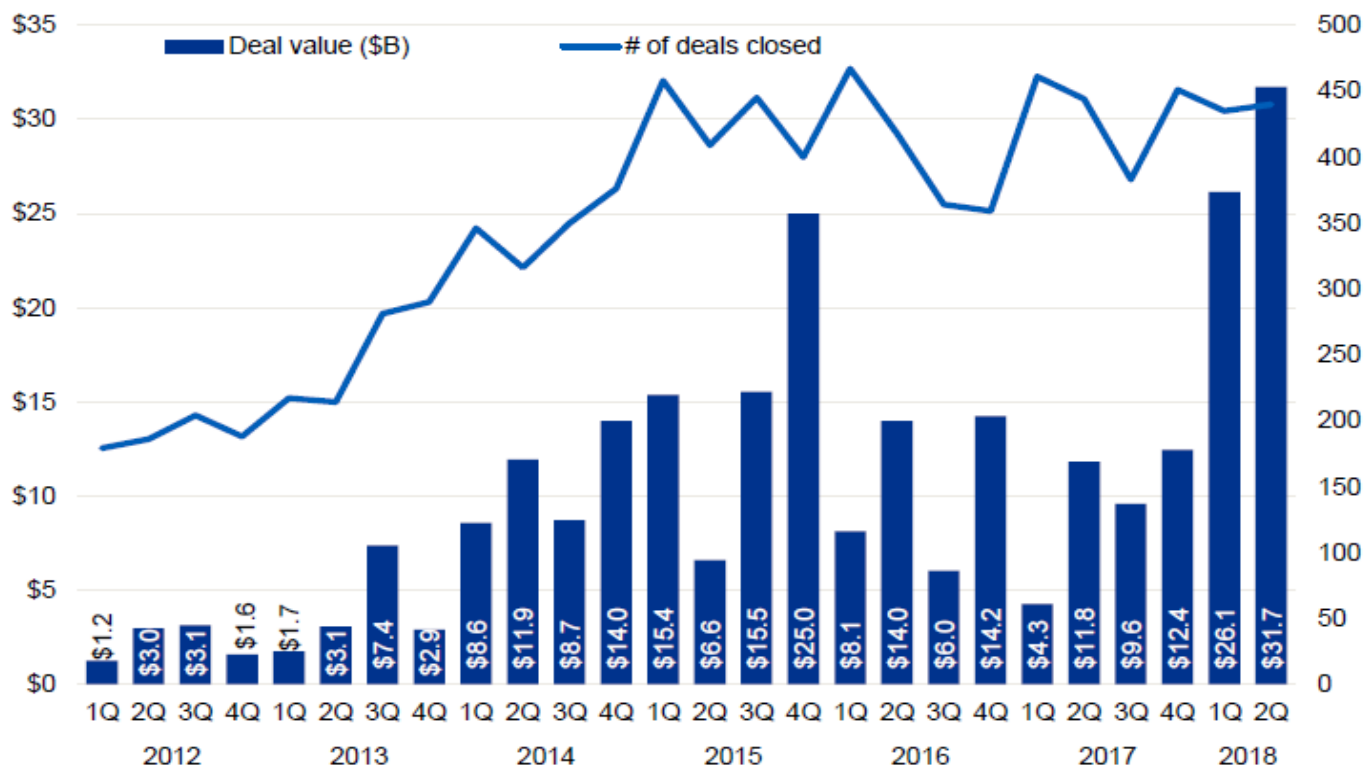
Global investment activity (VC, PE and M&A) in fintech companies 2012 – 30 June 2018
